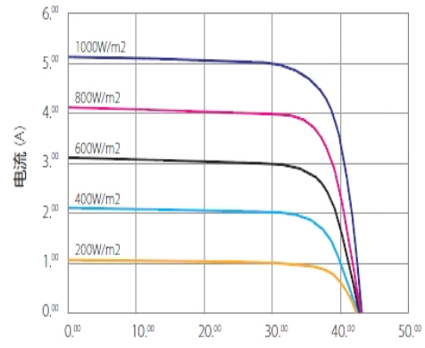
I-V Curve
