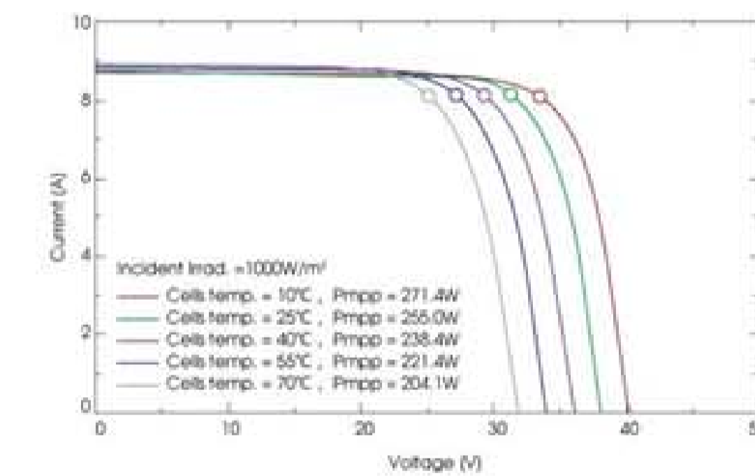
I-V Curves at different temperature
