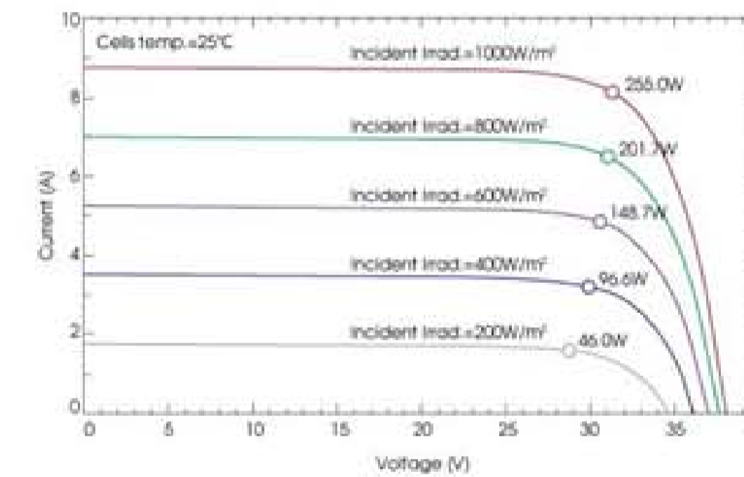
I-V Curves at different irradiance
