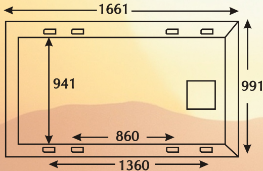
Module Back Side Schematic
