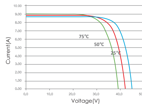
I-V Curves of PV Module GES-6M300 at Different Cell Temp. (AM1.5, 1000W/m 2 )
