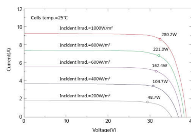
I-V Curves at different irradiance
