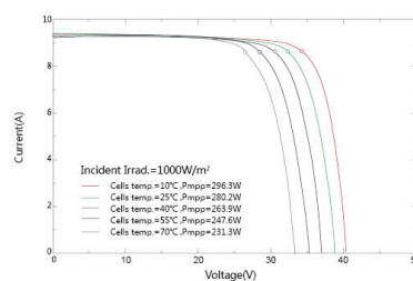
I-V Curves at different temperature
