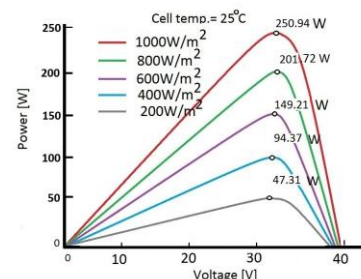
STC: Irradiance 1000W/m 2 , Module temperature 25°C, AM1, 5 spectrum
