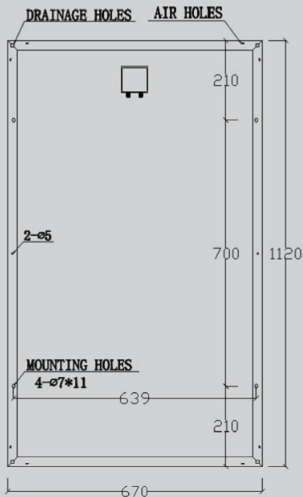
Engineering Drawings (Back Side)
