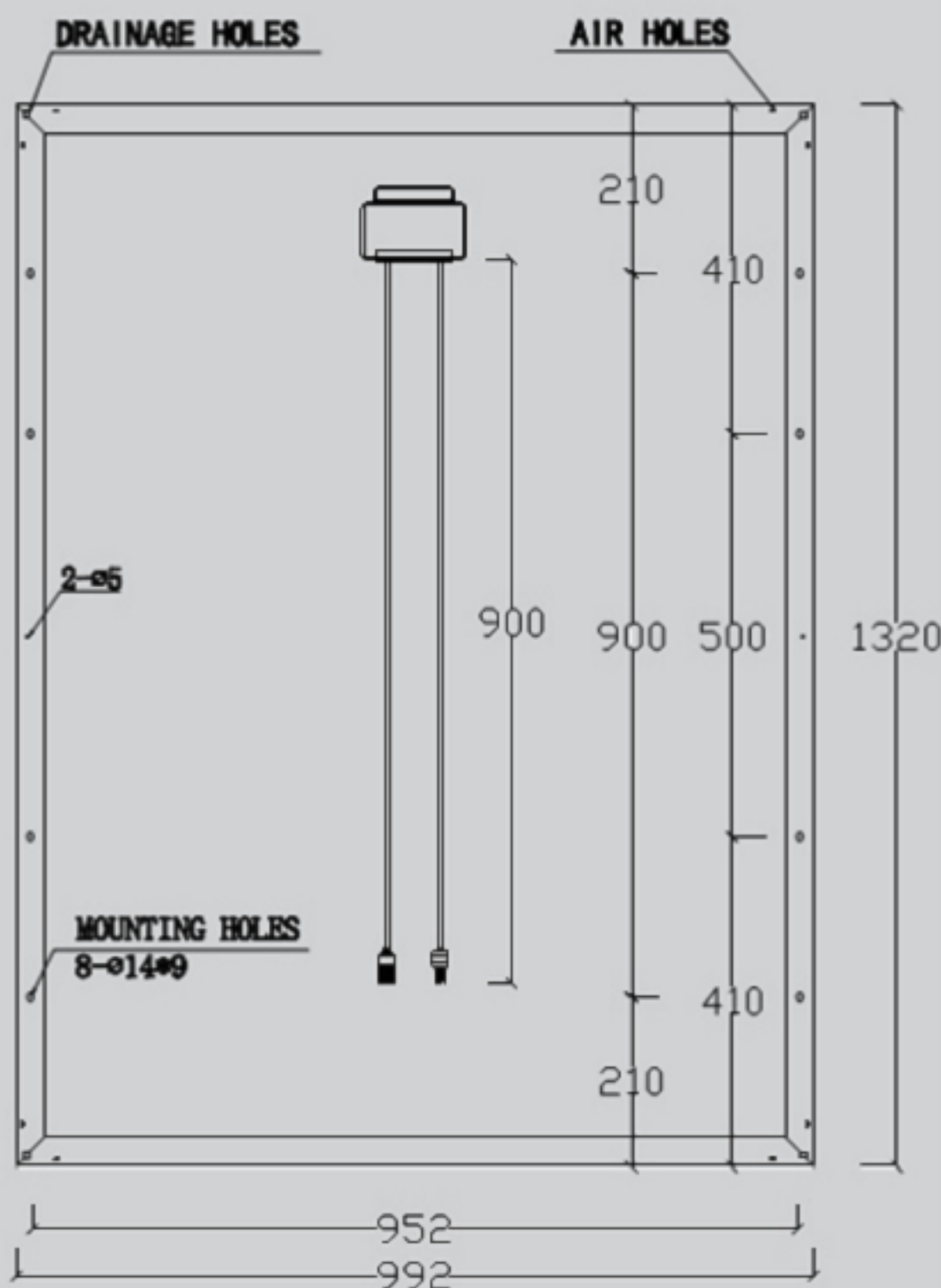
Engineering Drawings (Back Side)
