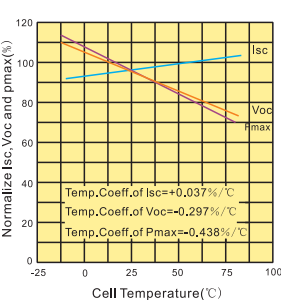
Temperature dependence of Isc, Voc and pmax
