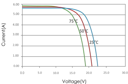
I-V Curves of PV Module SL5M36-90W at Different Cell Temp. (AM1.5, 1000W/m²)
