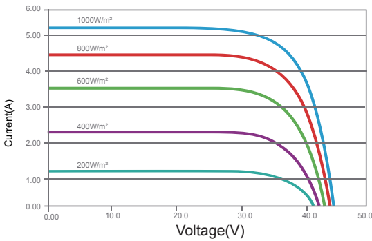
I-V Curves of PV Module PT5M72-190W (Cell Temp. 25 °C)
