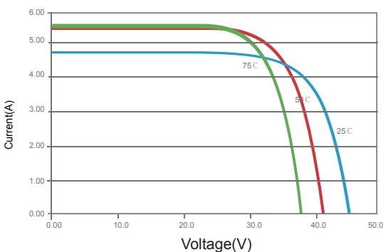
I-V Curves of PV Module PT5M72-190W at Different Cell Temp. (AM1.5, 1000W/m²)
