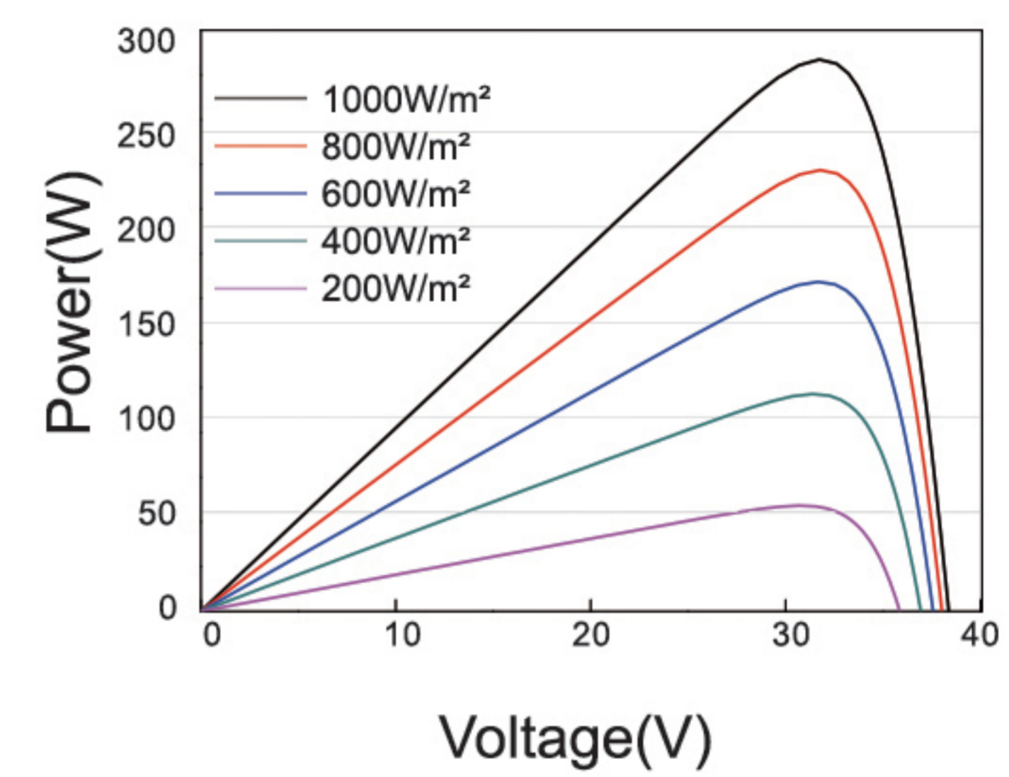
Power-Voltage Curve DHP60H-285
