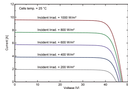
I-V Curve (SRP-365-BMA(-HV))
