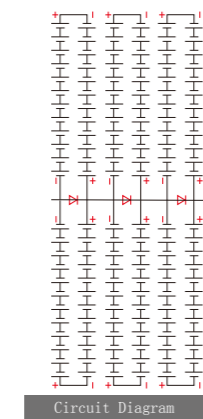
Circuit Diagram
