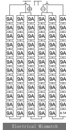
Electrical Mismatch
