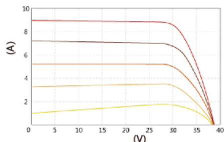
I-V Curve ( JY285M6-Ab-5 )
