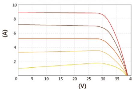
I-V Curve ( JY285M6-Ab-5 )
