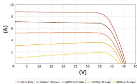
I-V Curve ( JY335M6-Aa-5 )
