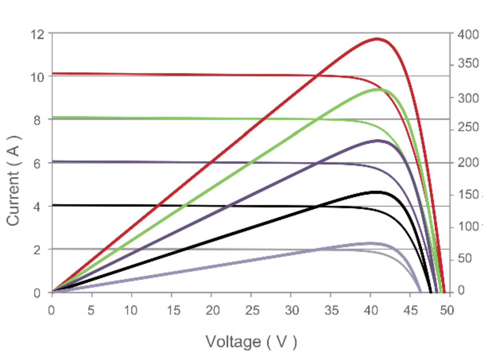
Current-Voltage & Power-Voltage Curves (390W)
