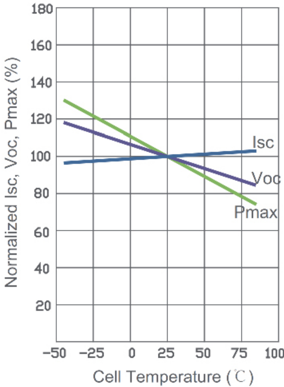
Temperature Dependence of Isc,Voc,Pmax
