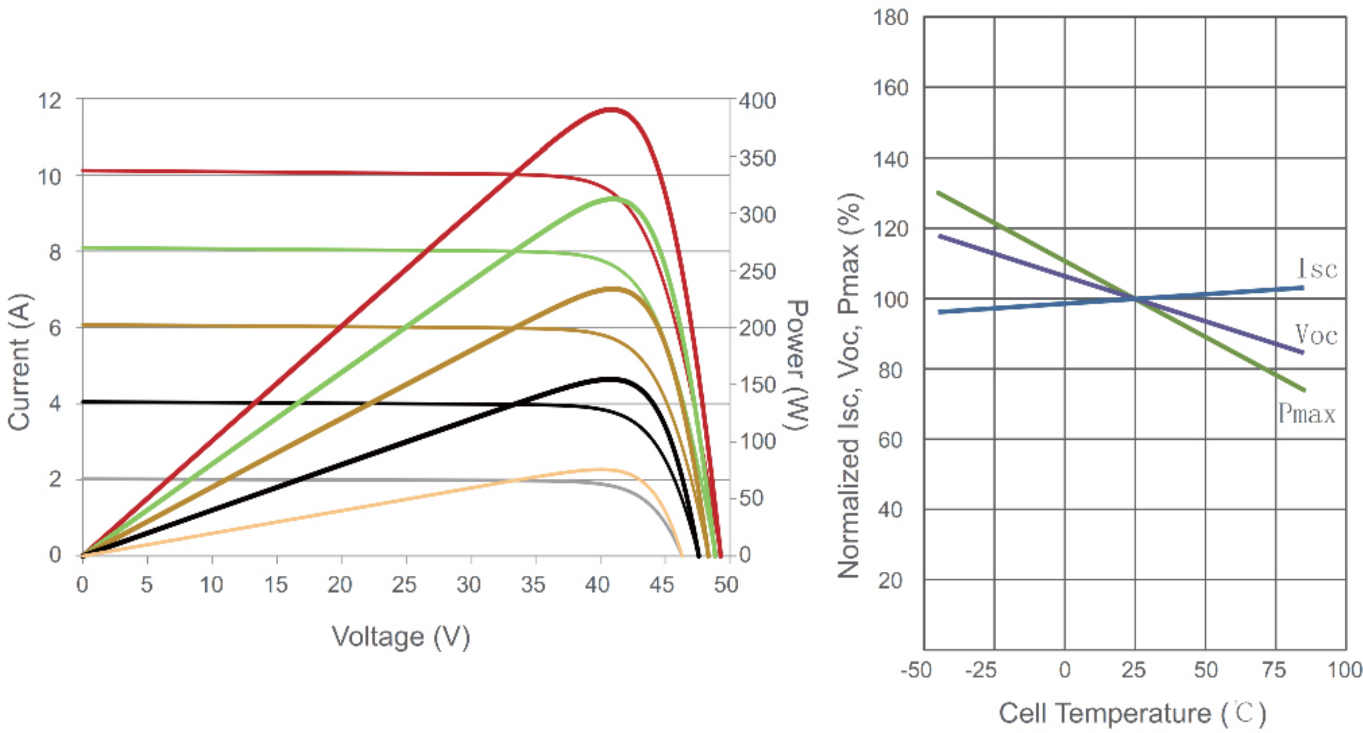
Current-Voltage & Power-Voltage Curves (390W) Temperature Dependence of Isc,Voc,Pmax
