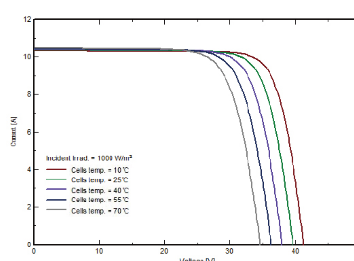
I-V Curve at different temperature (SPP320M60)
