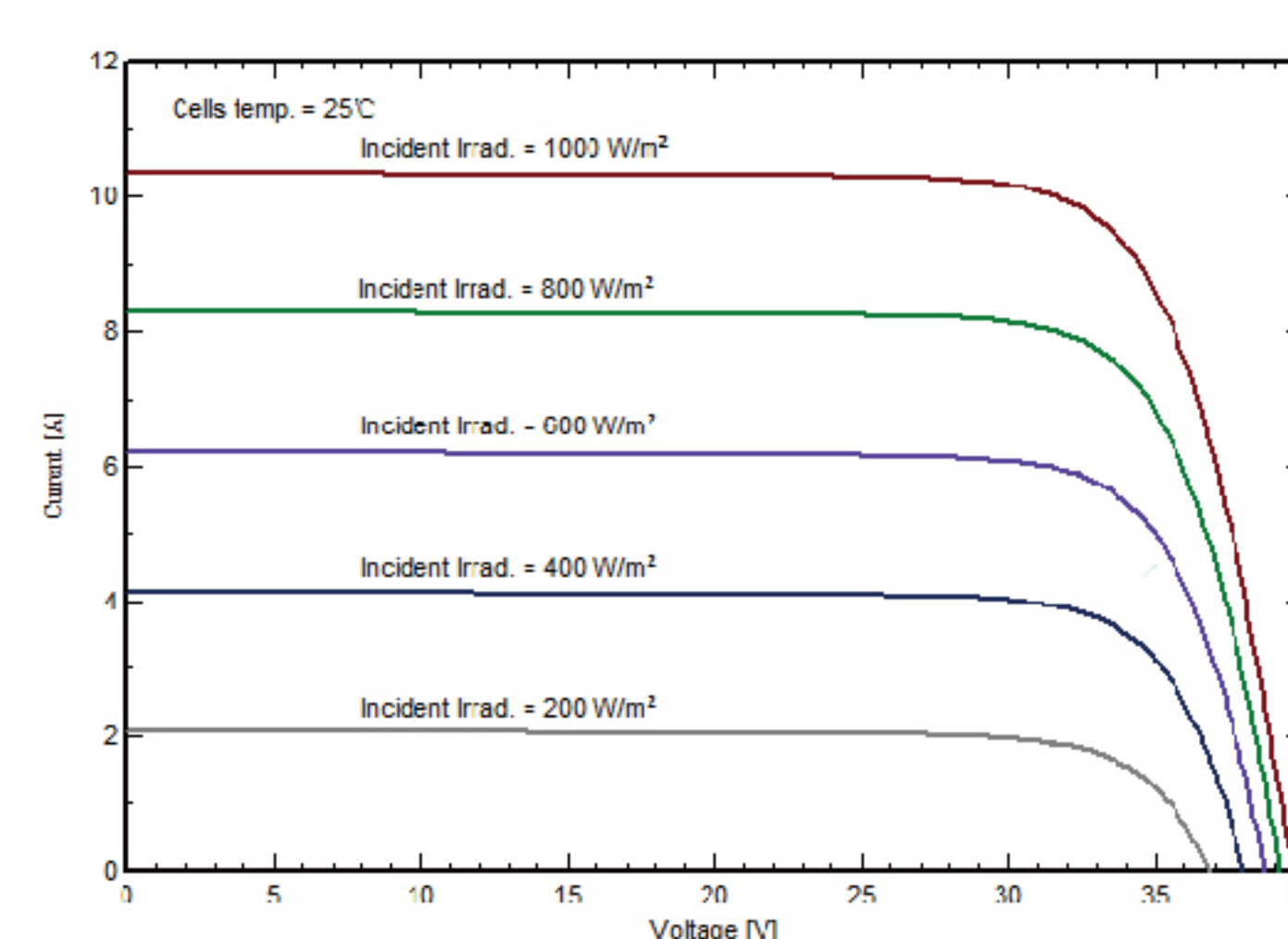
I-V Curve at different irradiation (SPP320M60)
