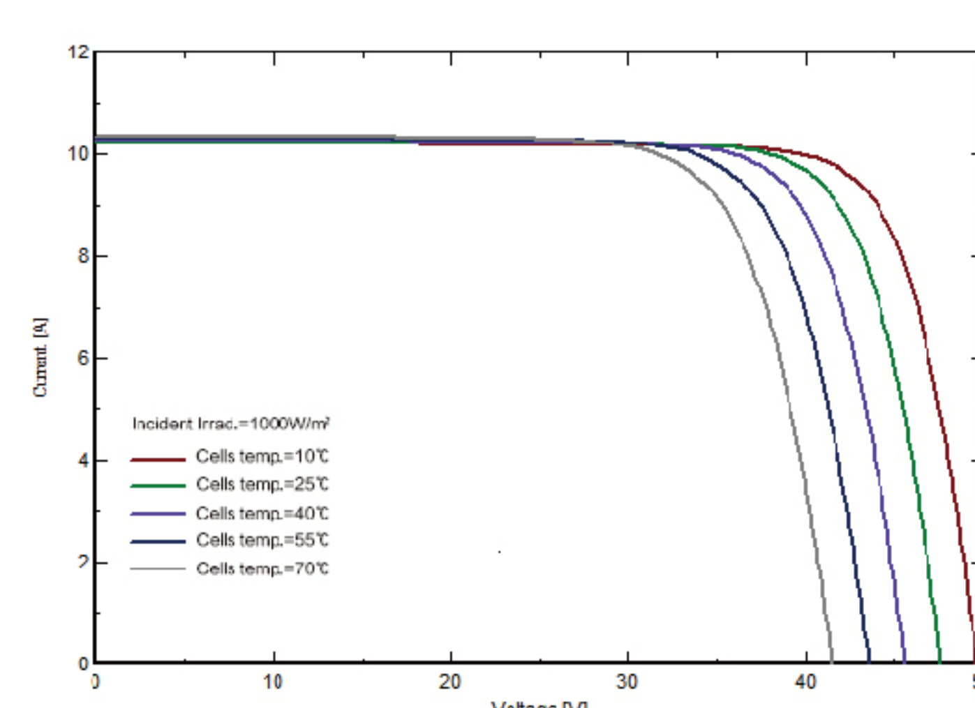
I-V Curve at different temperature (SPP385M72)
