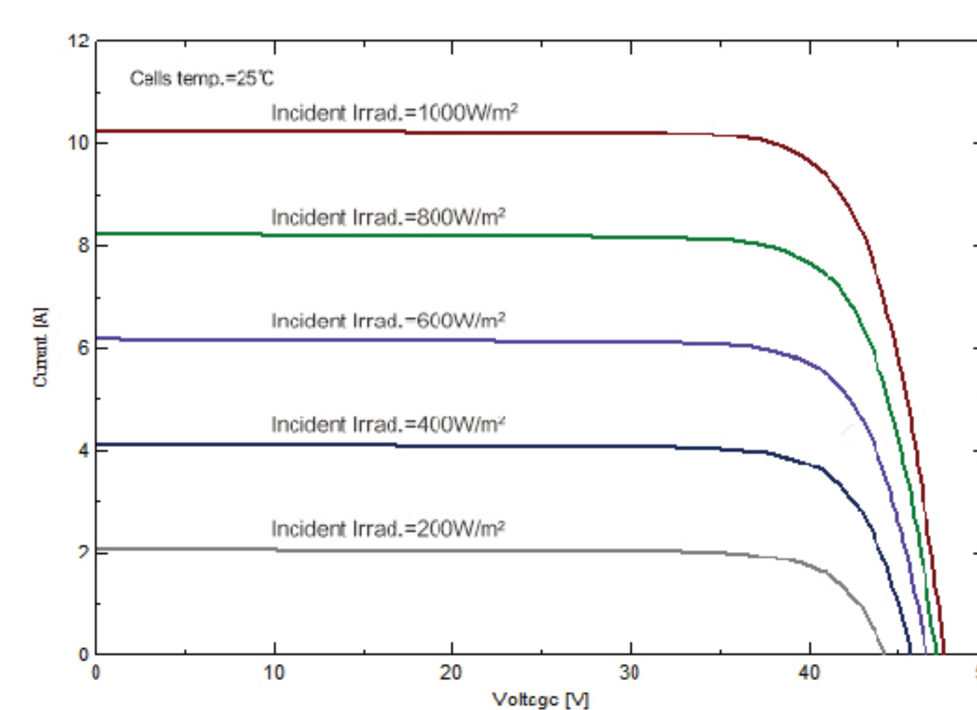
I-V Curve at different irradiation (SPP385M72)
