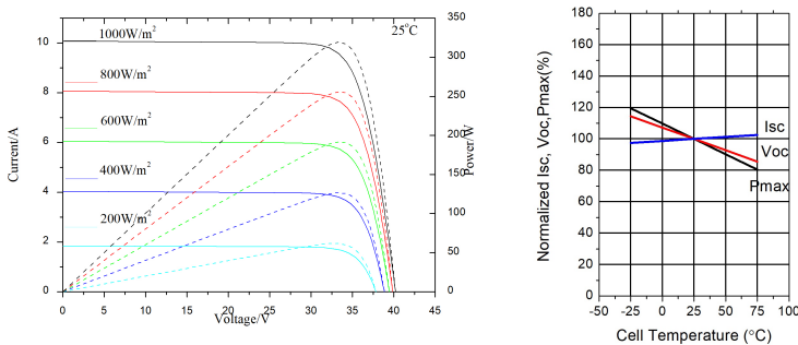
Electrical performance & temperature dependence Current-voltage & power-voltage curves (330W) temperature dependence of Isc, Voc, Pmax
