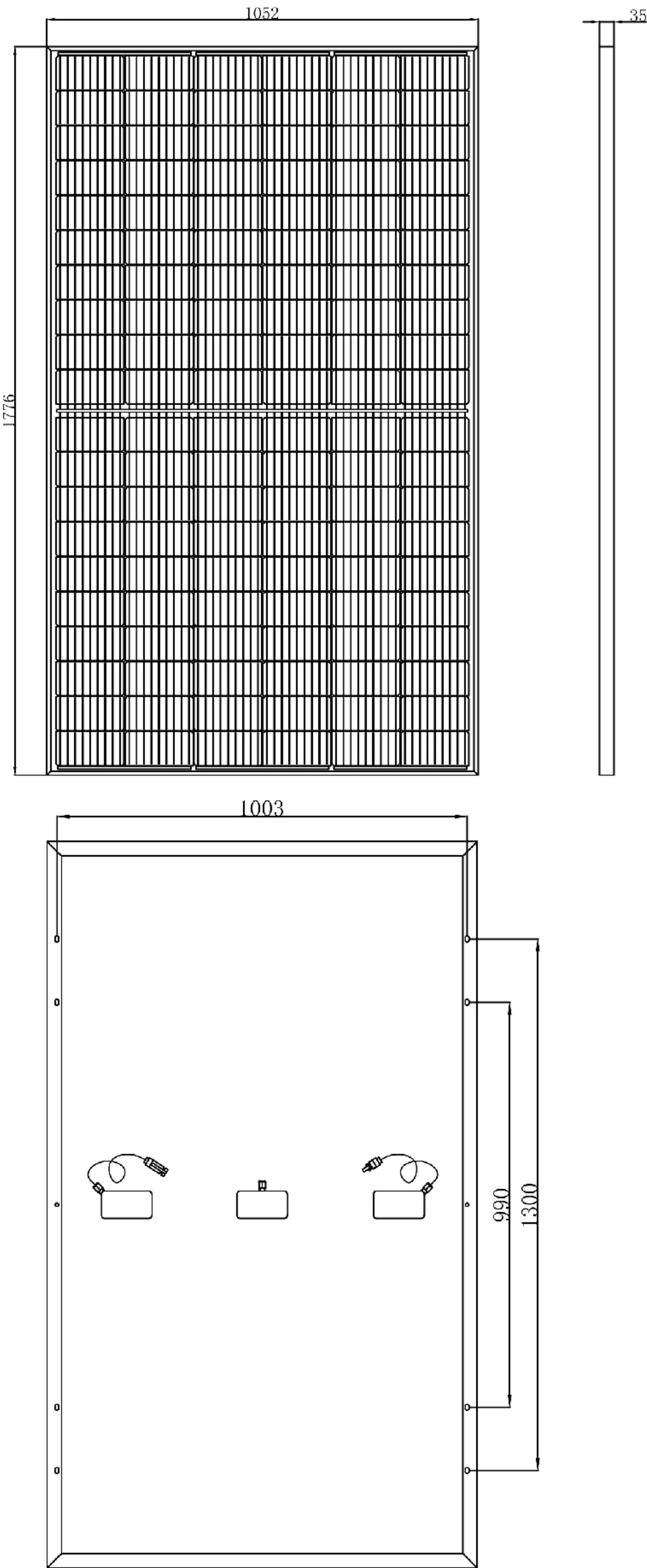
All Dimensions in mm(inch) The above drawing is a graphical representation of the product. For engineering quality drawings please contact SUNKET.
