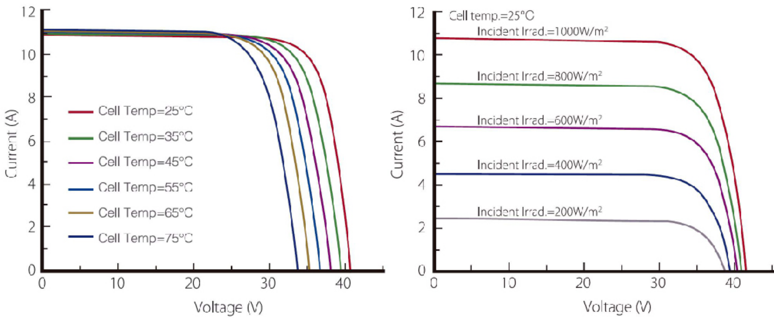
I-V Curve (SKT360M6-20)
