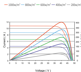
Current-Voltage & Power-Voltage Curves (410W)
