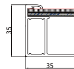
Section A-A Dimension (unit: mm)
