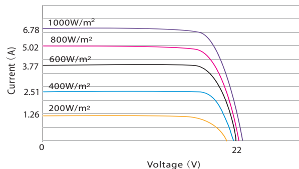
(SDM100-110) Current-Voltage Characteristic (I-V Curve)
