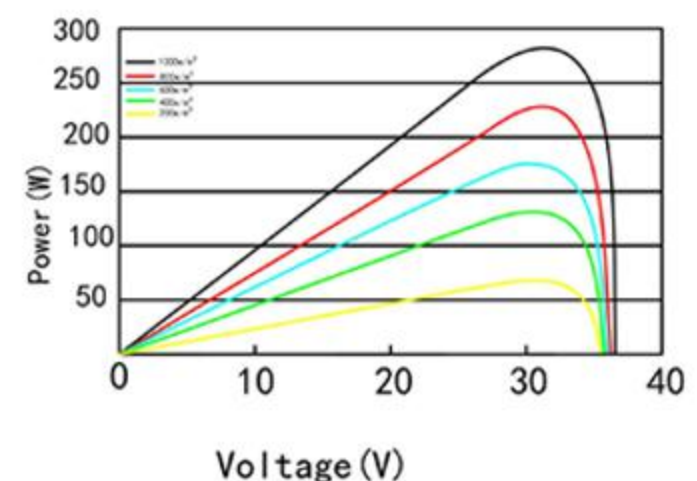
power-Voltage Curve
