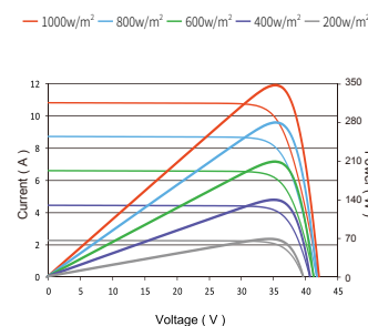
Current-Voltage & Power-Voltage Curves (350W)
