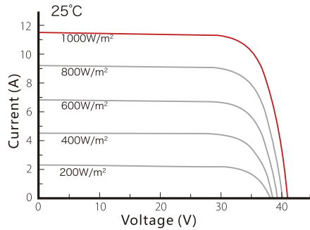
Power curve under different irradiance OLV-365-60M-DC6H
