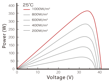
Power curve under different irradiance OLV-365-60M-DC6H
