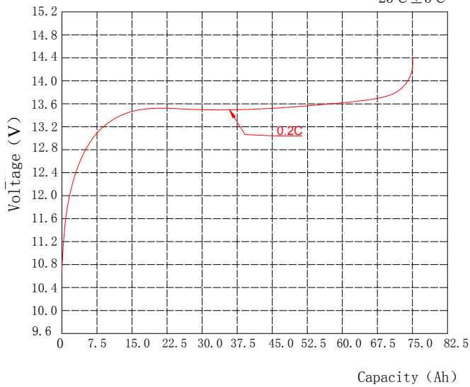
charge curve
