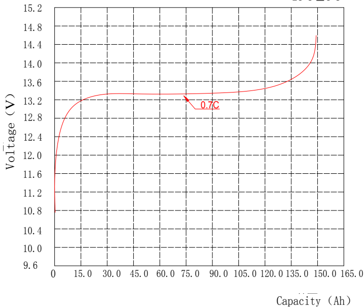
charge curve
