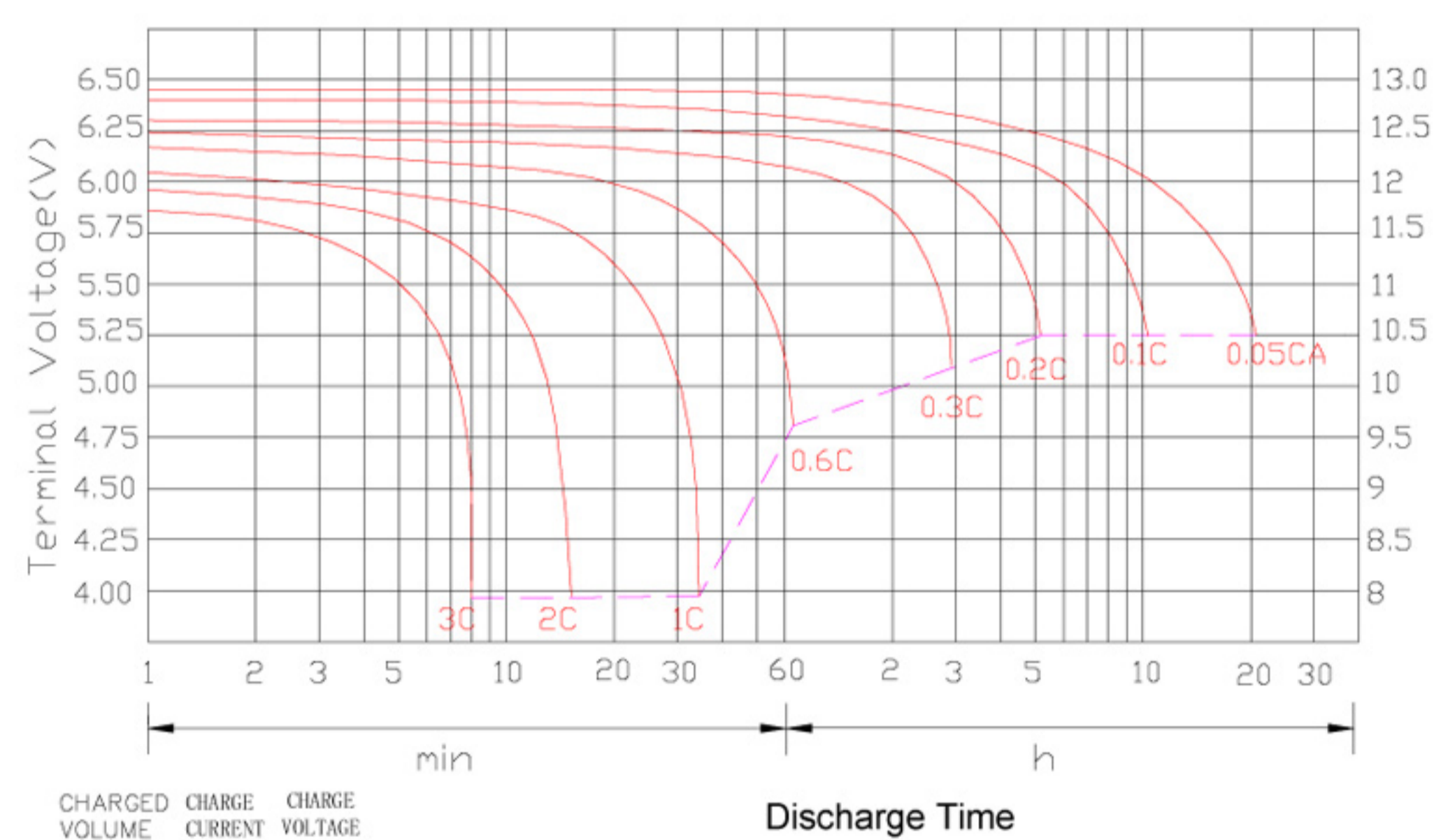
DISCHARGE CHARACTERISTICS AT 25° C(77° F)
