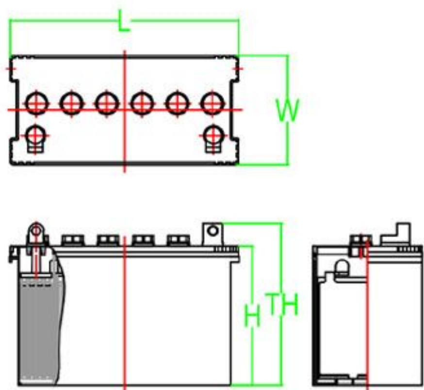
BATTERY LAYOUT
