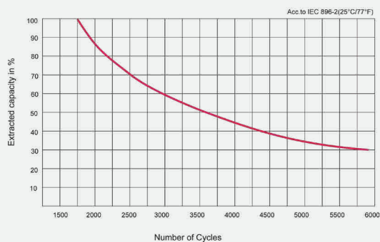
循环次数曲线 Cycle Life Characteristics
