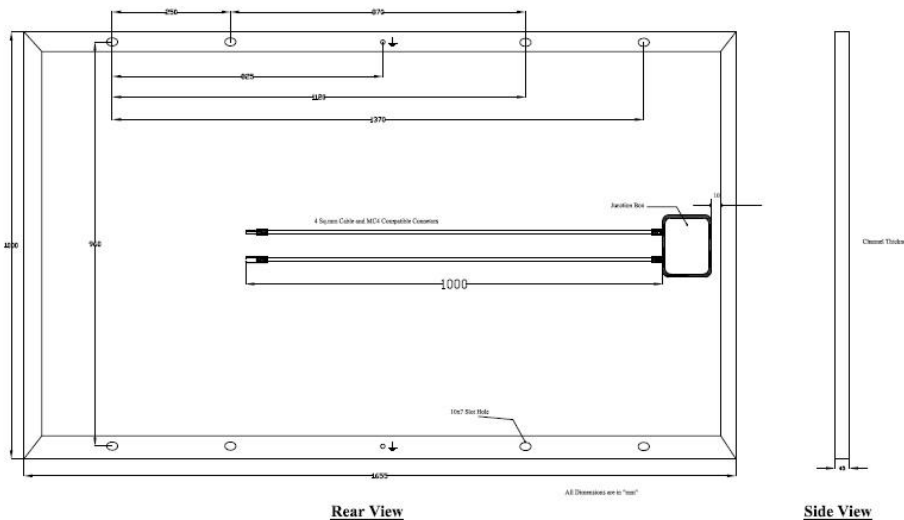
245Wp PV Module Dimension Details
