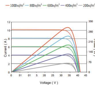
Current-Voltage & Power-Voltage Curves (310W)
