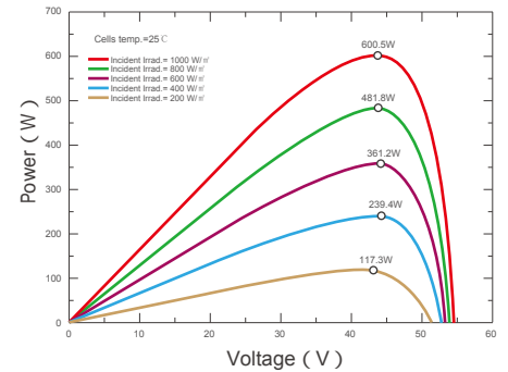
Current-Voltage &amp; Power-Voltage Curves (SKT600M10)
