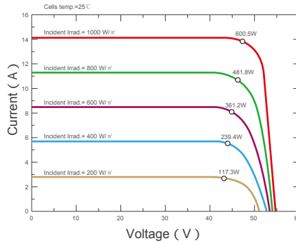
Current-Voltage &amp; Power-Voltage Curves (SKT600M10)
