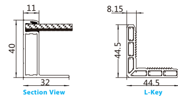
Section View
