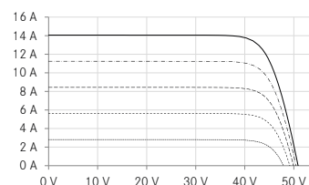
UI - diagram e.g. 560 Wp
