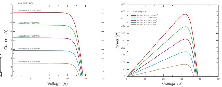
Current-Voltage & Power-Voltage Curves (SKT430M10-108D4)
