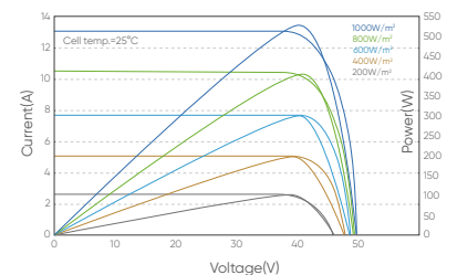
I-V/P-V Curve at Different Irradiation (555W)
