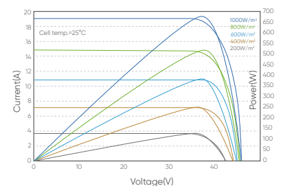
I-V/P-V Curve at Different Irradiation (675W)
