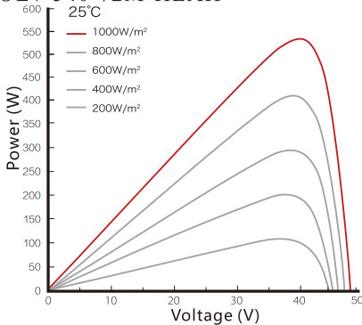
Power curve under different irradiance OLV-540-72M-HEAH
