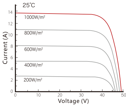
I-V Curves at Different Irradiances OLV-540-72M-HEAH
