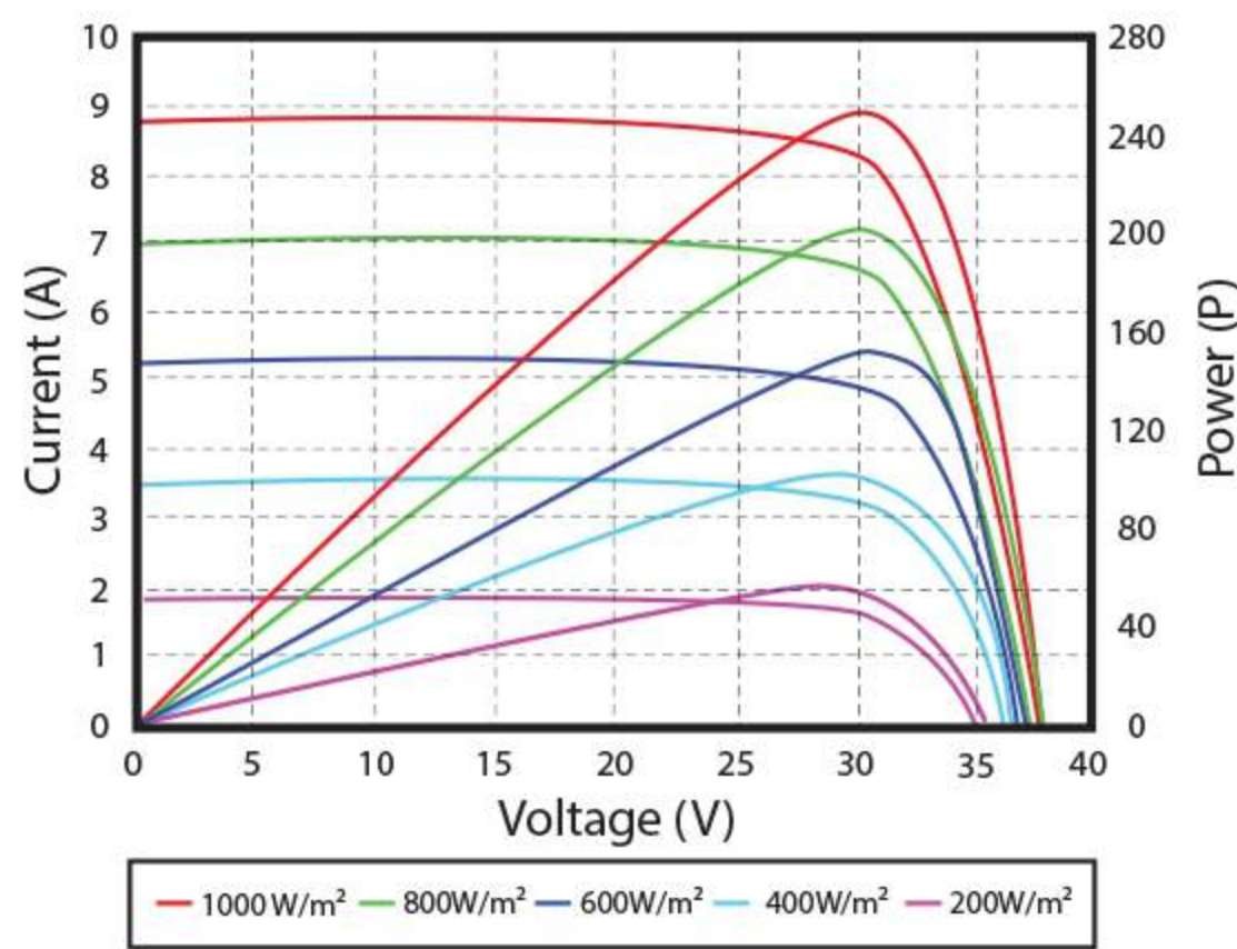
Current-Voltage and Power-Voltage Curves at Different Irradiances
