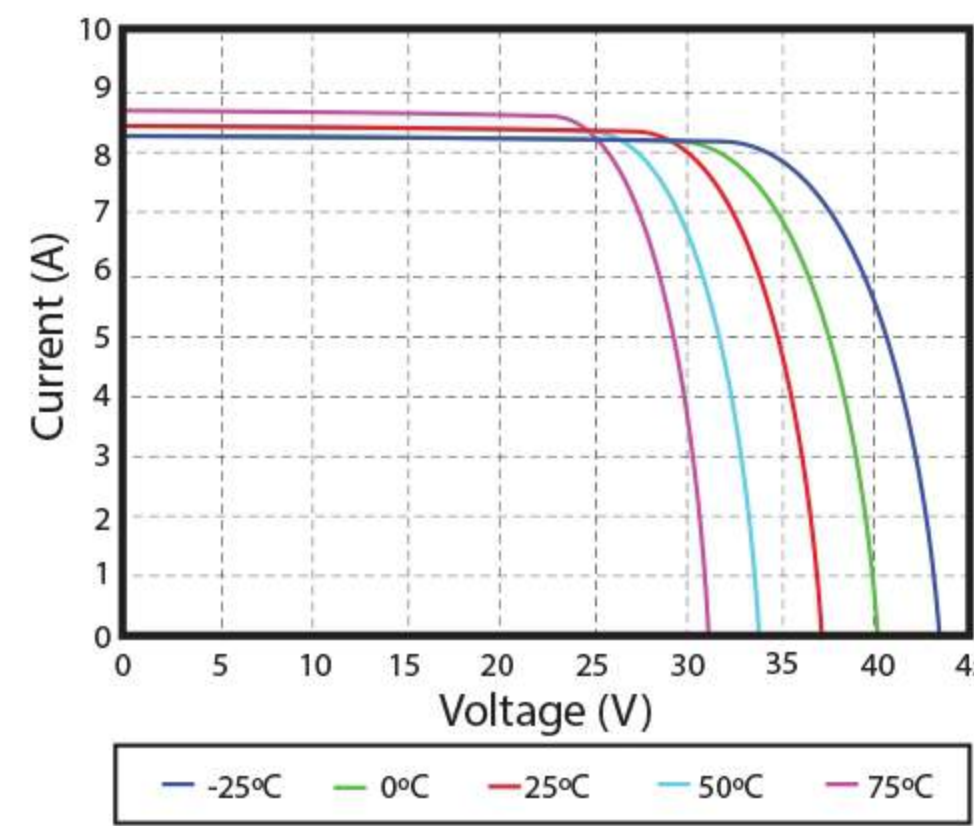
Current-Voltage Curves at Different Temperatures
