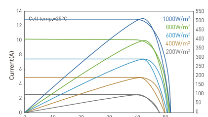
I-V/P-V Curve at different Irradiation (500W)
