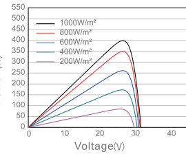
Power Voltage Curve SP400M/32
