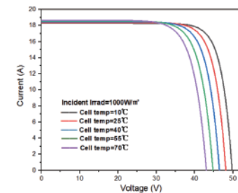
I-V characteristics at different temperatures (SP-N18/132HG 700W)
