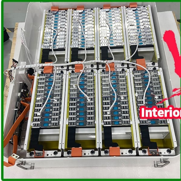
PKNERGY -- Laser Welding
