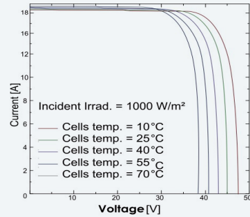
I-V / P-V CURVE AT DIFFERENT TEMPERATURE (680W)
