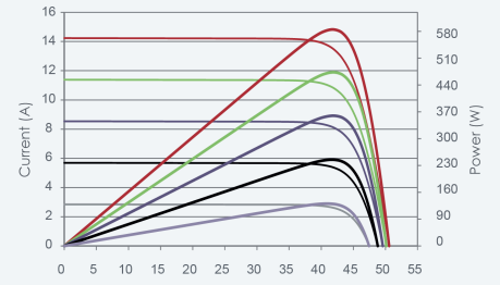
Current-Voltage & Power-Voltage Curves (580W)
